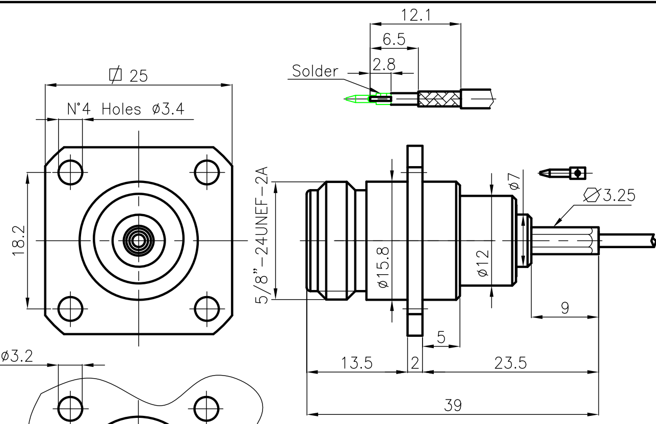
PANEL CUTOUT DIMENSIONS
