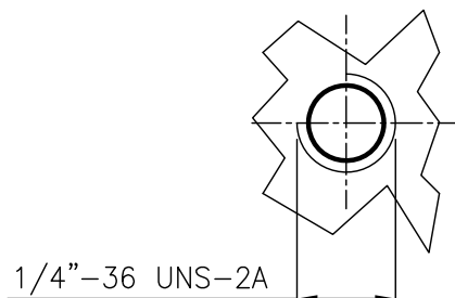
PANEL CUTOUT DIMENSION
