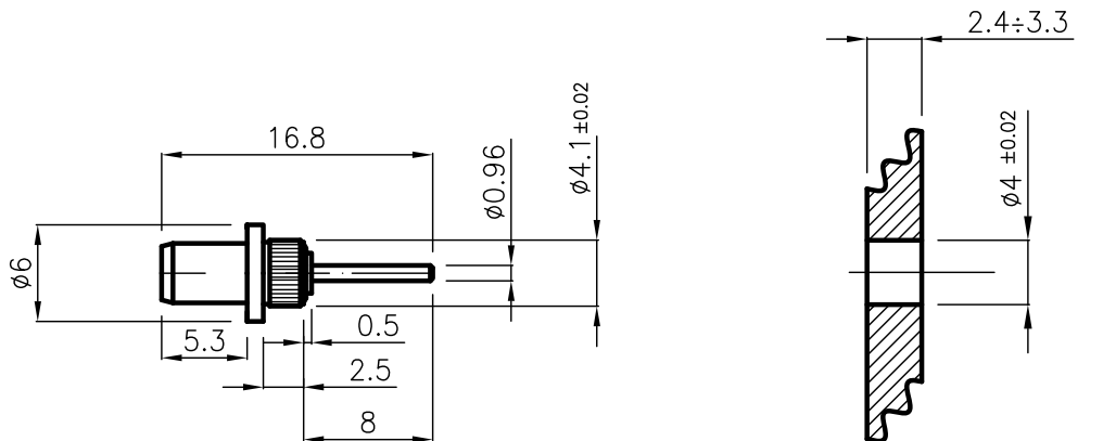
MOUNTING HOLE
