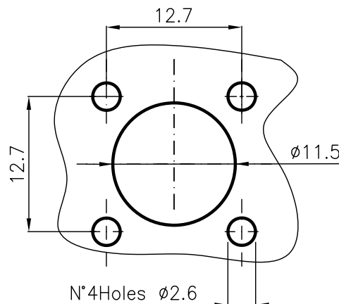
FRONT PANEL - CUTOUT DIMENSIONS
