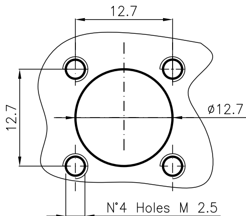
REAR PANEL - CUTOUT DIMENSIONS
