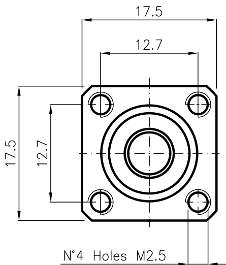
REAR PANEL - CUTOUT DIMENSIONS
